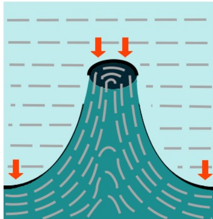
(b) Pillar formation
