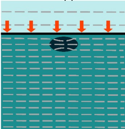
(a) Shock approach
