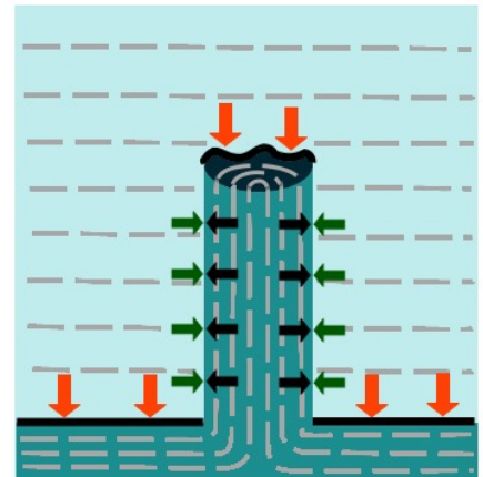
(c) Pillar erosion
